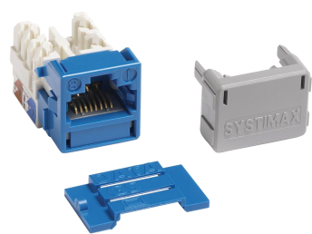
GigaSPEED XL® MGS400 Series Category 6 U/UTP Information Outlet, blue
